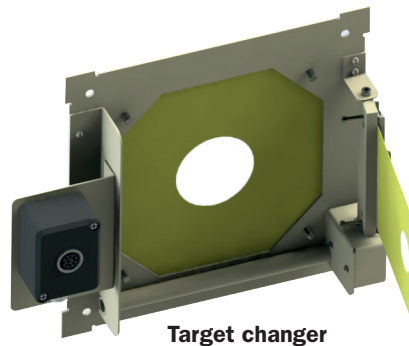
Target changer
